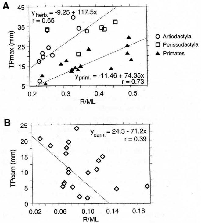
Figure 11.6. Least squares regression plots of R standardized by mandibular length (ML) against (A) TP max in primates, perissodactyls, and artiodactyls; and (B) TP carn in carnivores.
