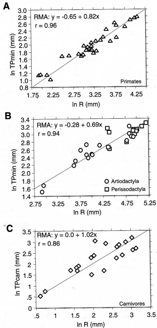
Figure 11.5. Reduced major axis regression of log-transformed R versus TP_{\min} . (A) Primates. (B) Combined herbivore sample (artiodactyls and perissodactyls). (C) Carnivores. The slopes of the primate and herbivore regressions but not the carnivores are significantly different from isometry ( P < 0.001 ).
