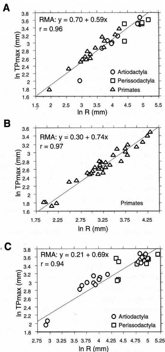
Figure 11.4. Reduced major axis regression of log-transformed R versus TP_{\max} . (A) Combined sample of primates and ungulate herbivores; (B) primates; (C) combined herbivore sample (artiodactyls and perissodactyls). The slopes of the primate and herbivore regressions are not significantly different from each other but both are significantly different from isometry ( P < 0.001 ).
