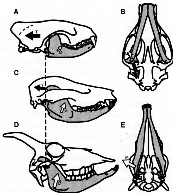
Figure 11.1. Comparison of TMJ and cranial morphology in mammals with ginglymoid and diarthroidal TMJs. (A, B) Lateral and inferior views of a mustelid ( Martes pennanti ) with a ginglymoid TMJ. Note the TMJ lies in the same plane as the postcanine occlusal plane; the dominant adductor is the temporalis, T; the superficial masseter, M, is small, in a parasagittal plane, and anteriorly oriented. The sizes of the arrows indicate schematically the relative size of the temporalis versus the masseter and medial pterygoid complex. (C) Lateral view of opossum ( Didelphis virginianus ) in which the short diarthroidal TMJ lies slightly above the occlusal plane; the temporalis and masseter muscles are roughly equivalent in size; the masseter is more laterally and dorsally oriented than in the carnivore. (D, E) Lateral and inferior views of a goat ( Capra hircus ). Note the tall ramus, which positions the occlusal plane well below the long diarthroidal TMJ; the temporalis is small relative to the size of the masseter. The masseter has a strong dorsal and lateral orientation, whereas the medial pterygoid has a dorsal and medial orientation.
