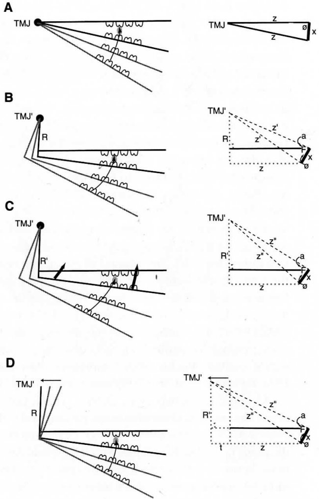
Figure 11.2. Geometric model of TMJ function in relation to occlusal plane position. (A) Ginglymoid TMJ in which the orientation of the mandibular tooth row relative to the maxillary tooth row, \phi , at any given gape, x , equals \arccos(X/2Z) . (B) Effect of positioning the occlusal plane below the TMJ by distance R so that \phi = \Phi - \alpha (see text for details), introducing an anterior component to the trajectory of the mandibular teeth relative to the maxillary postcanine occlusal plane. (C) Effect of increasing ramus height to R' , which makes \phi more acute relative to the postcanine maxillary occlusal plane (see text for details). Note also that \phi is more anteriorly oriented (thick arrows) for more posterior teeth that lie closer to the TMJ. (D) Effect of posterior translation on the orientation of the mandibular tooth row relative to the maxillary tooth row, making \phi more dorsally oriented.
